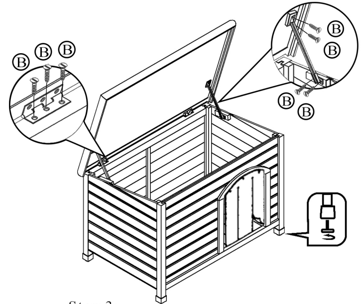
Step 3: Secure roof onto the body
